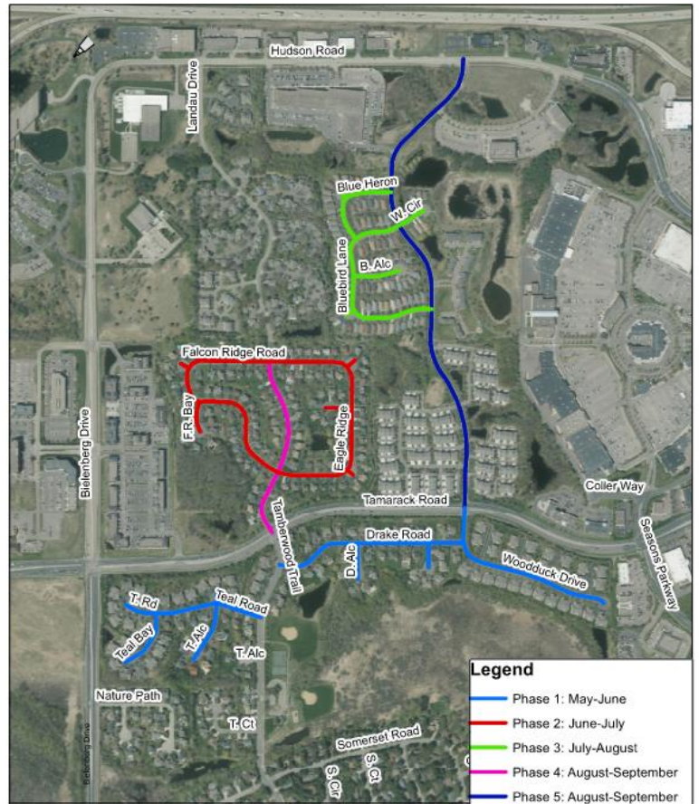
2021 ROADWAY REHABILITATION PROJECT PHASING MAP
