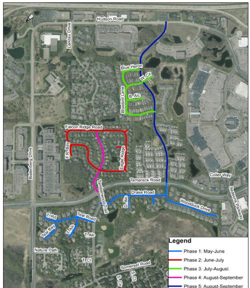
2021 ROADWAY REHABILITATION PROJECT PHASING MAP
